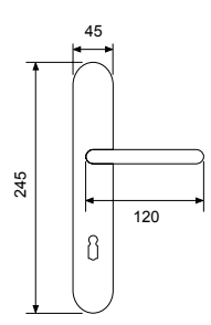
21016P - OCS Handle on plate Maner cu placa
