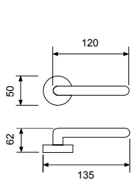
21058R03 - OBG Handle on rose Maner cu rozeta
