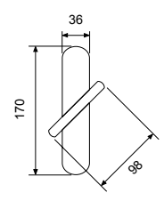
20292 - OLV Window handle Cremon
