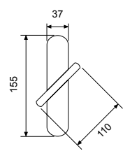
2058 - OBG Window handle Cremon
