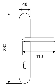
21023P - OLV Handle on plate Maner cu placa
