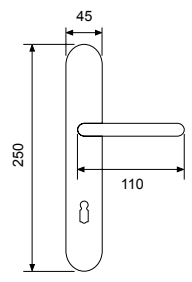
21034P - OBG Handle on plate Maner cu placa
